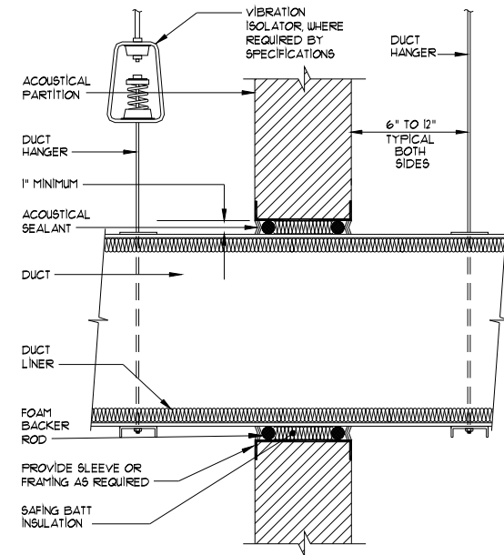
4 TYPICAL DUCT PENETRATION THROUGH ACOUSTICAL PARTITION
